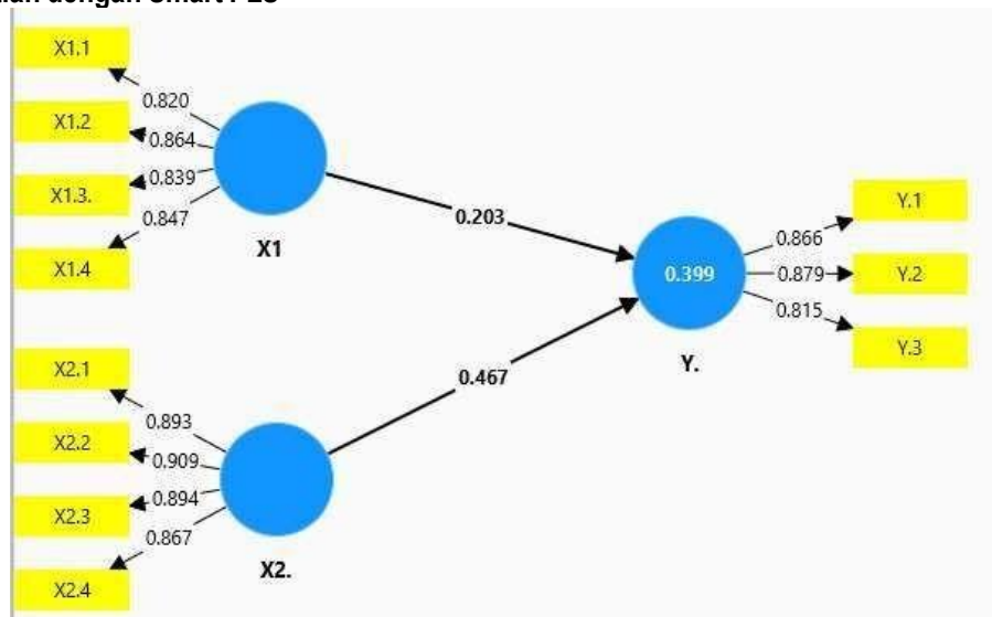
Gambar 3. Output PLS
