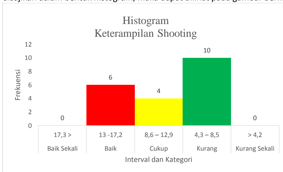
Gambar 1. Histogram Keterampilan Shooting
