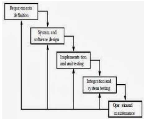
Gambar 1. Waterfall Model
