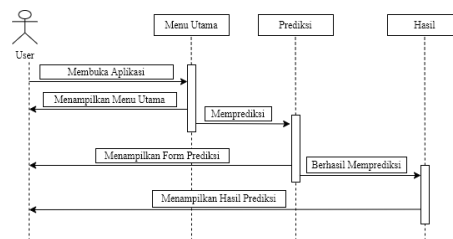
Gambar 3. Sequence Diagram
