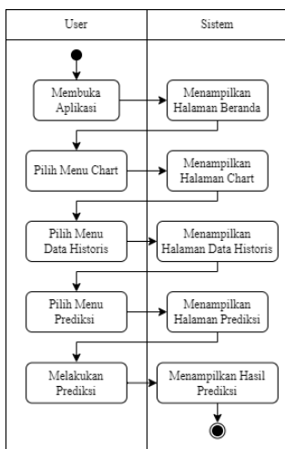
Gambar 4. Activity Diagram
