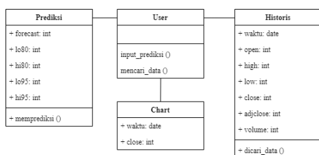
Gambar 5. Class Diagram
