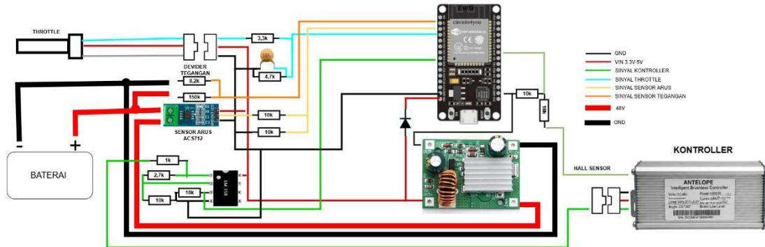
Gambar 2. Wiring Diagram
